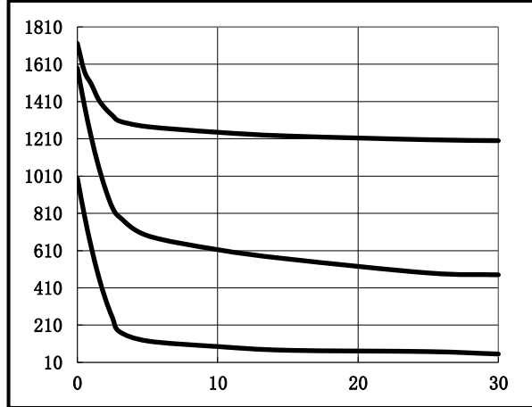
Fig.2 Capacitance Characteristics
